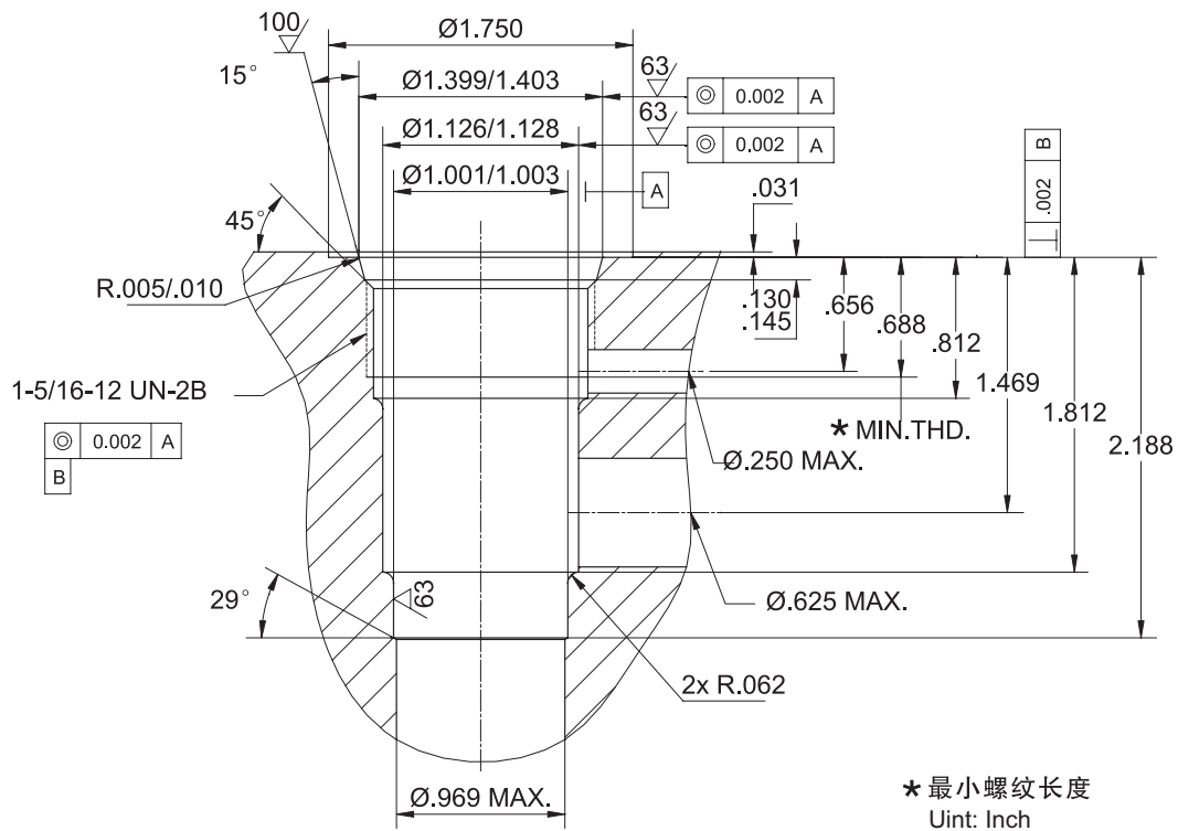
CAVITY:16-S3
