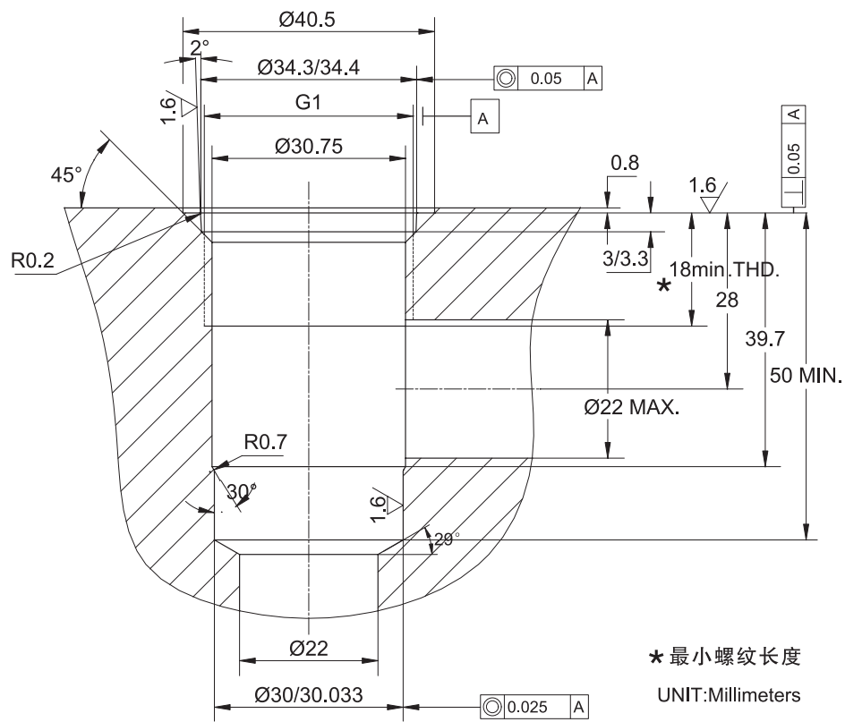
CAVITY:16S-2
